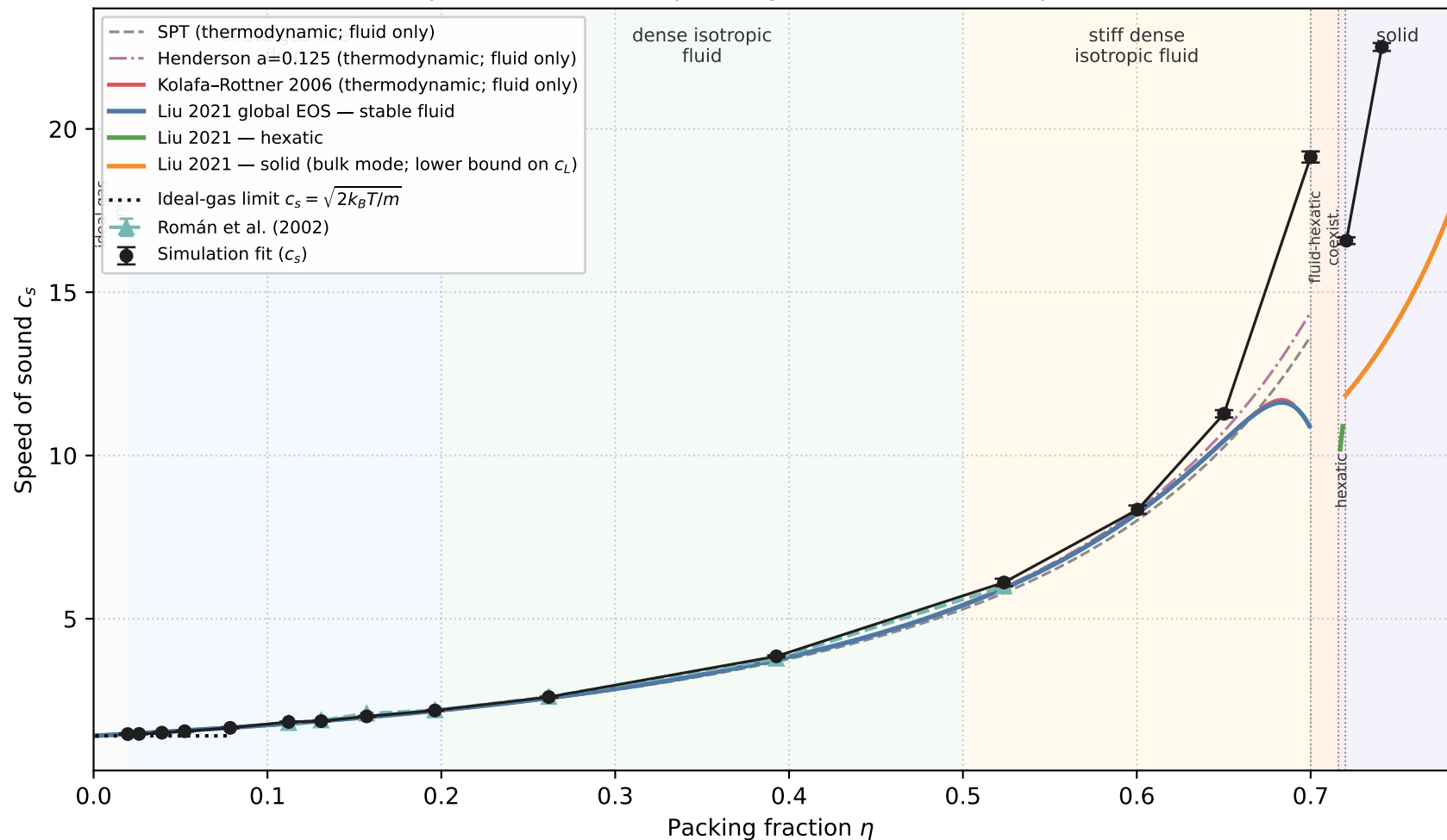
Hard disks: speed of sound vs packing fraction (r11 c25, phase-aware EOS)
